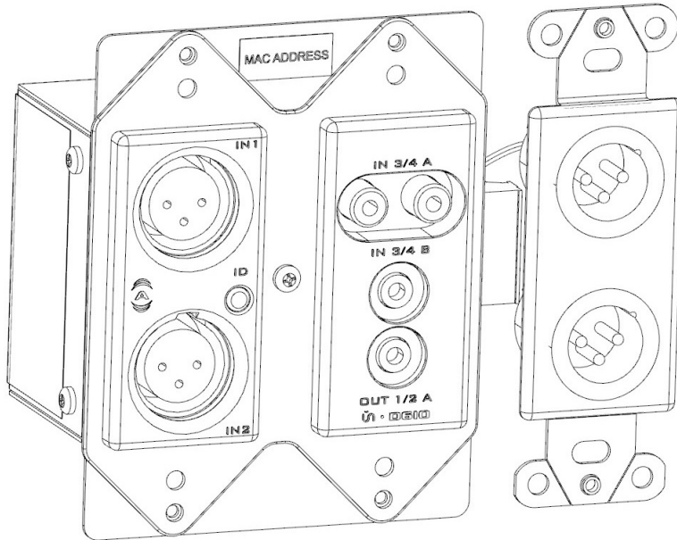
Figure 3 - unD6IO with unXP20 Plate (Front)
