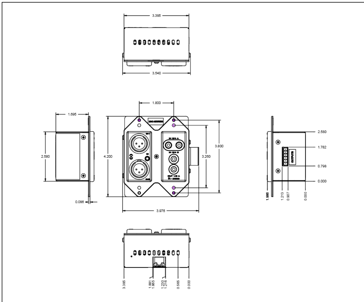
Figure 5 - Dimensioned Drawing
